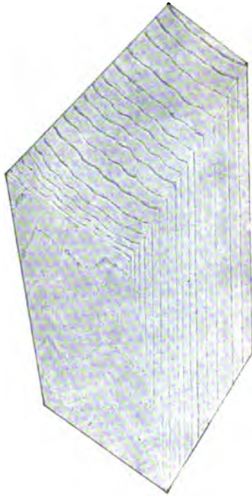
Fig. 26.—Type of Cypress-wood ( Chamaecyparis , Cupressus , Thuja , Libocedrus , Juniperus , etc.).
